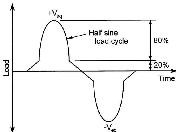
Fig. 9.3—Permitted approximation of alternating seismic-shear cycle.
